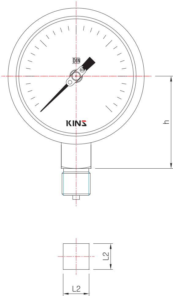
Model No. | SF-3021 (100mm) A Type (Rimless type)
